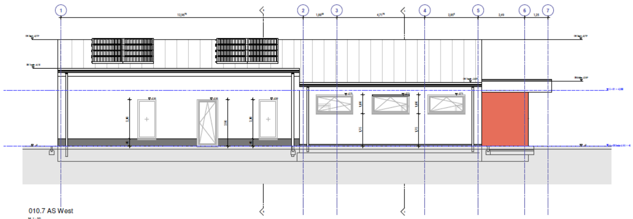
010.7 AS West M 1:50
